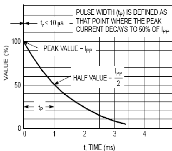
Figure 2. 10 x 1000 μs Pulse Waveform
